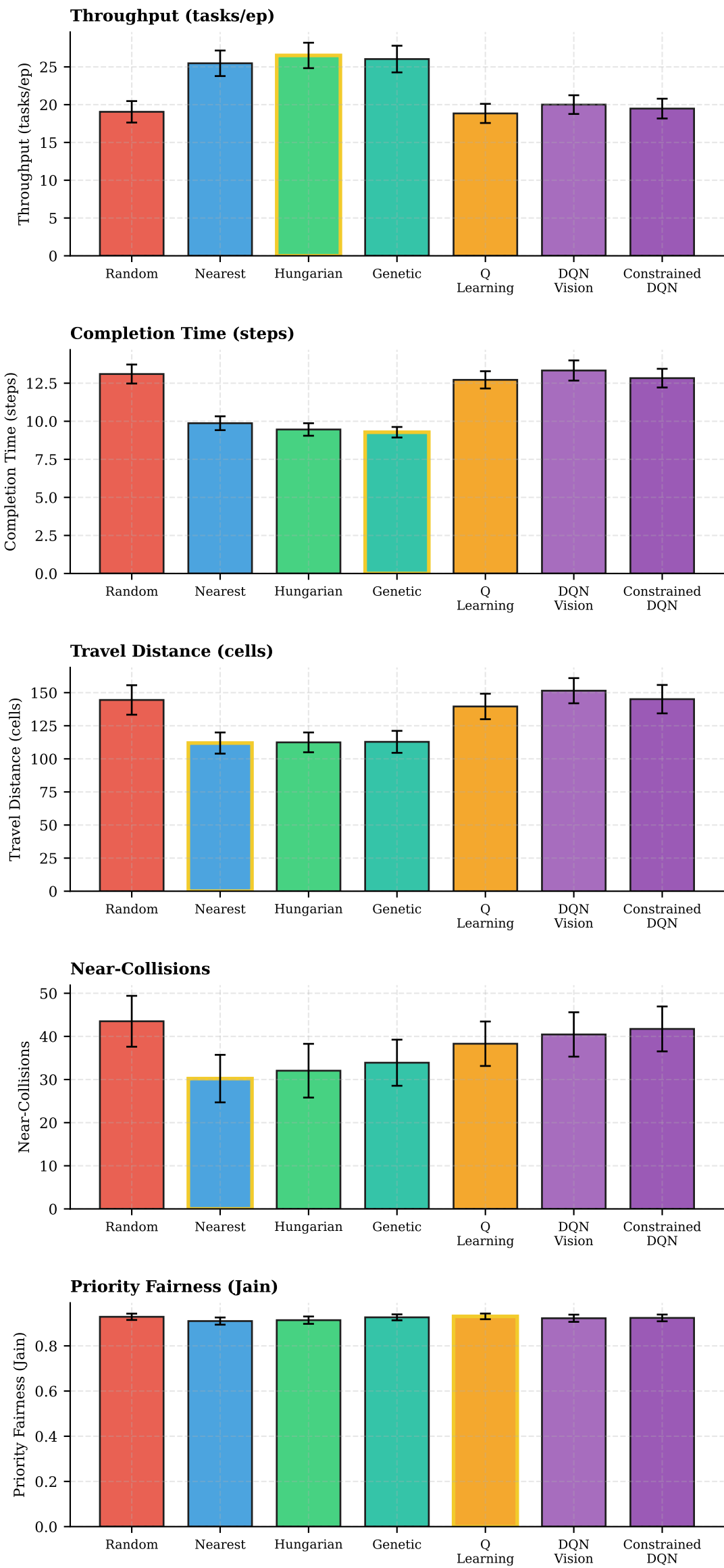
Fig. 4: Algorithm Comparison Across Logistics KPIs
