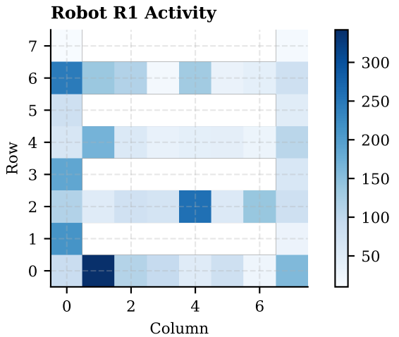
Fig. 11: DQN-Vision Spatial Activity Heatmaps
