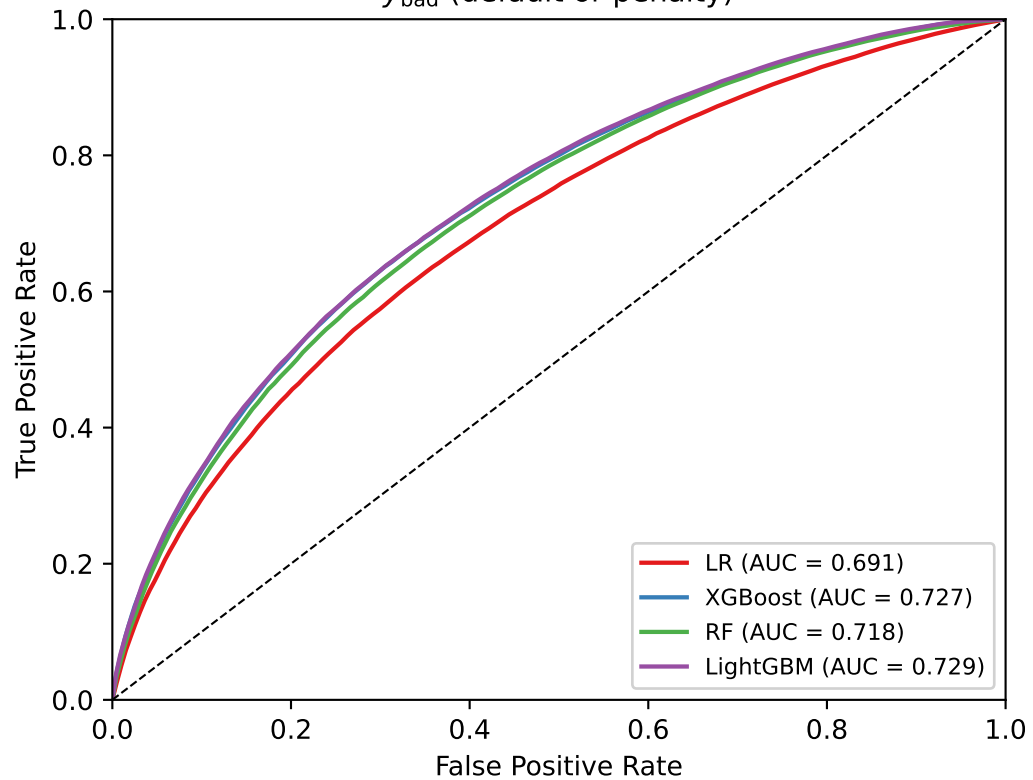
y_{\text{bad}} (default or penalty)
