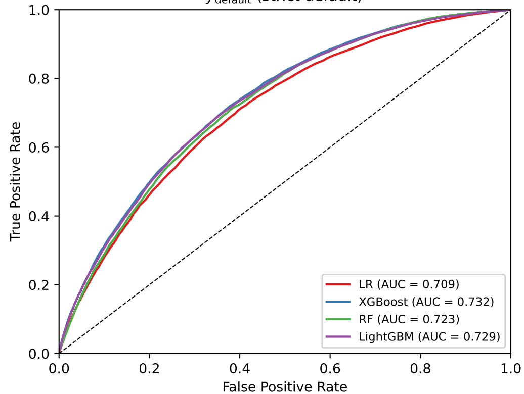
y_{\text{default}} (strict default)
