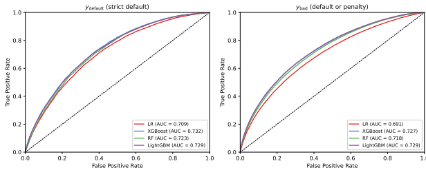
Figure 1. Out-of-fold ROC curves for all four classifiers on both prediction targets ( n = 222,618 , 5-fold OOF). AUC values match Table 2.
