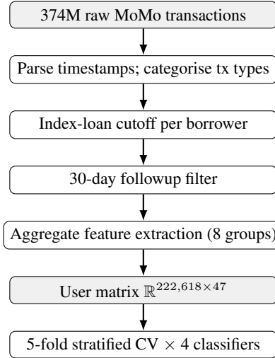
Figure 2. End-to-end pipeline from raw transactions to cross-validated model evaluation.
