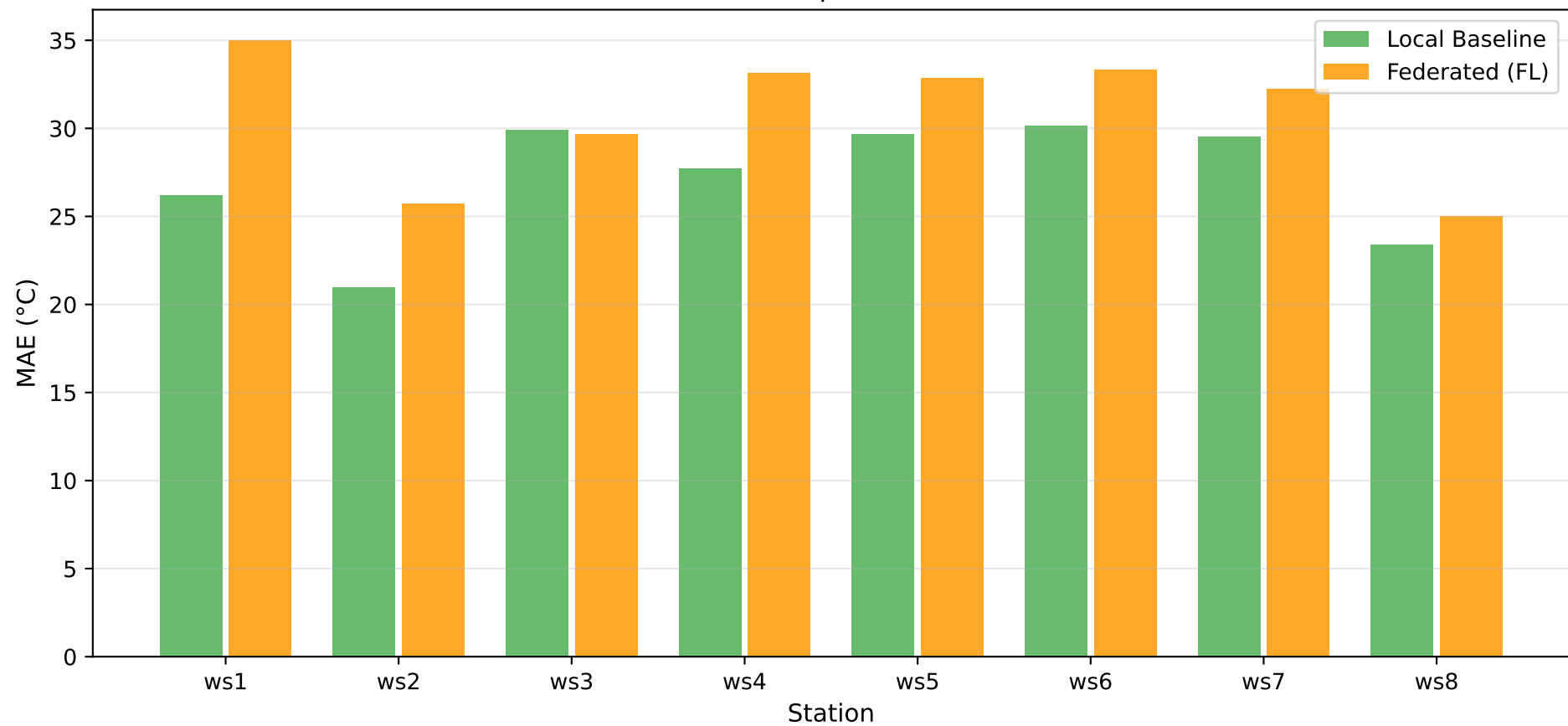
Per-Station MAE Comparison — Crossformer
