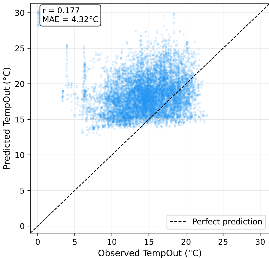
Predicted vs Observed — Crossformer Centralised
