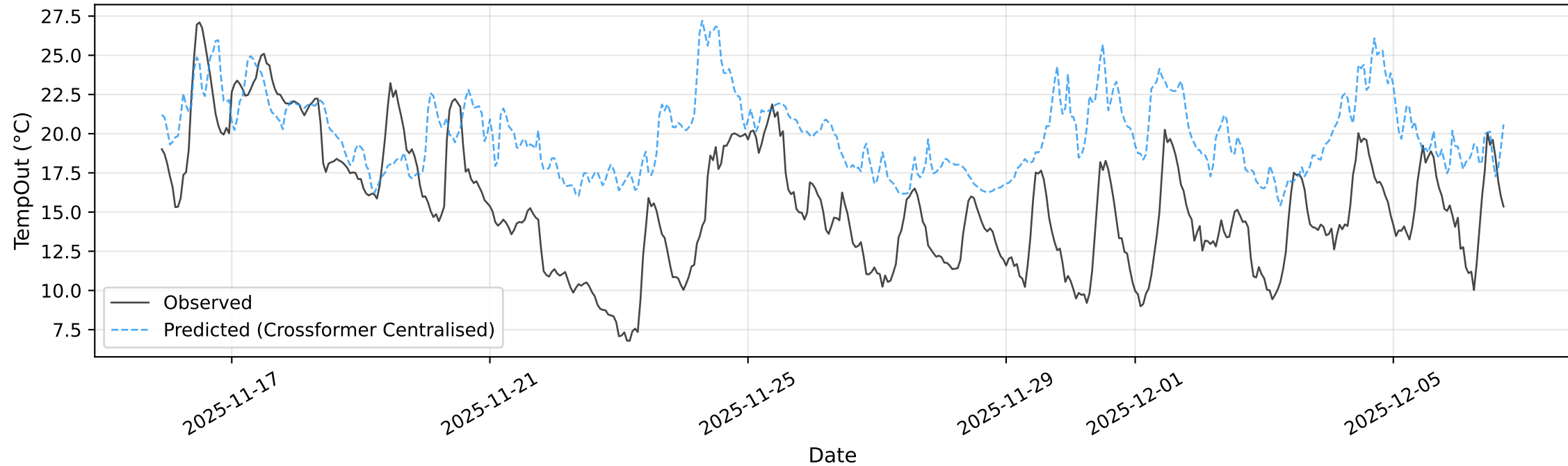
Observed vs Predicted — ws1 — Crossformer Centralised (test set, first 500h)
