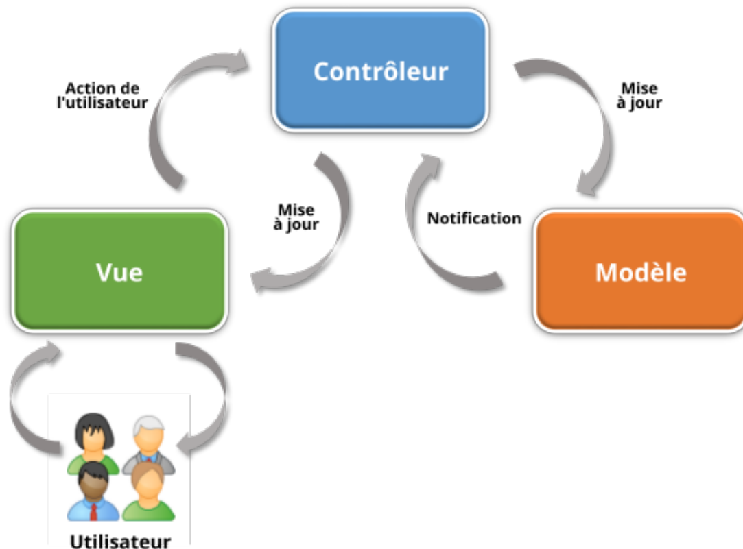
Figure 2.1: Architecture MVC [?]
