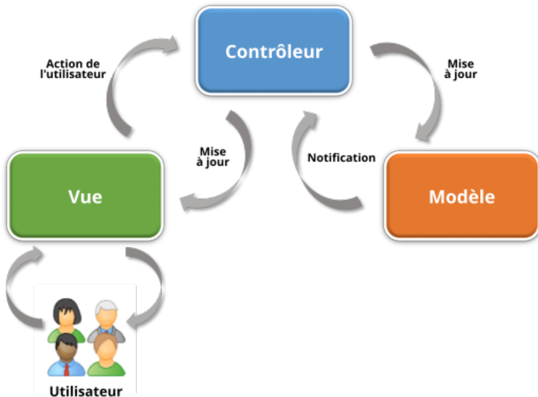
FIGURE 2.1 : Architecture MVC [10]
