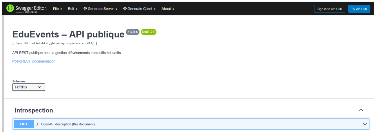
FIGURE 4.1 : API swagger 1
