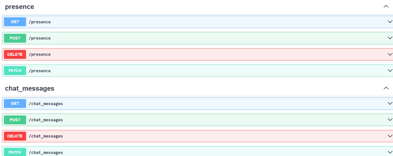
FIGURE 4.3 : API swagger 3
