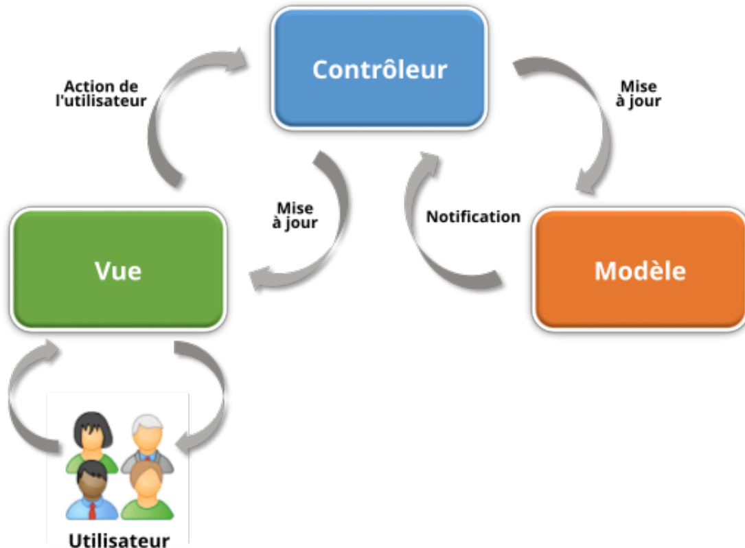
FIGURE 3.1 : Architecture MVC [9]
