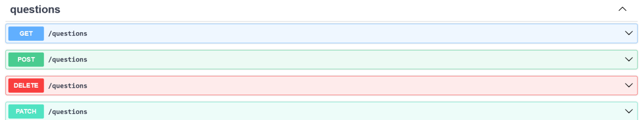
FIGURE 3.5 : API swagger 5
