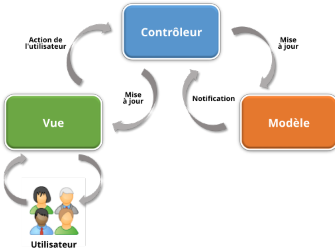
FIGURE 2.1 : Architecture MVC [10]
