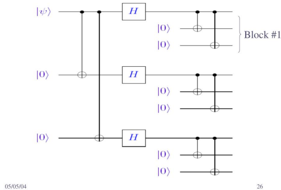
Figure 16: shor code の回路図
