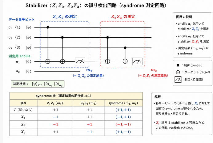
Figure 17: Stabilizer 測定回路
