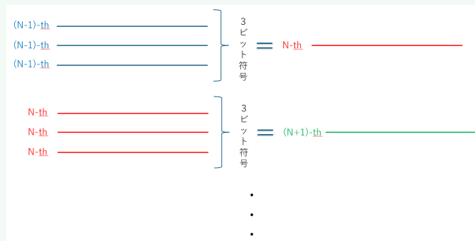
Figure 21: 入れ子構造
