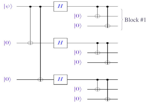
Figure 16: shor code の回路図
