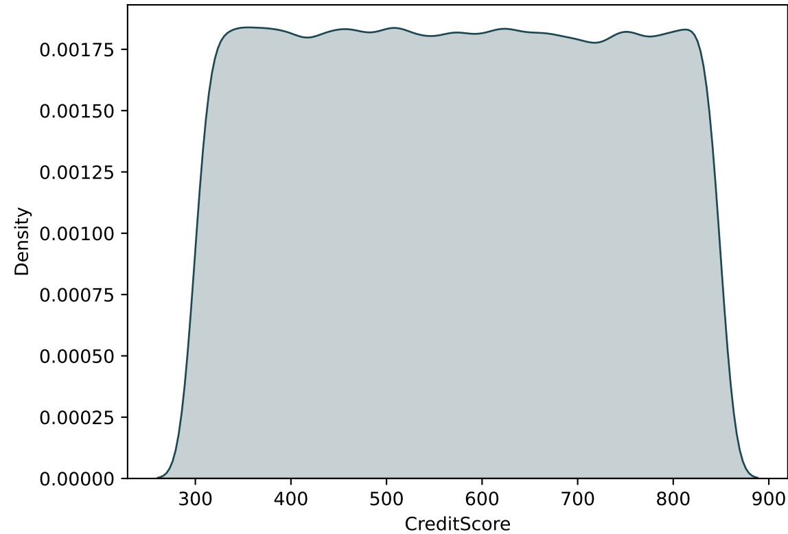
Distribution of CreditScore
