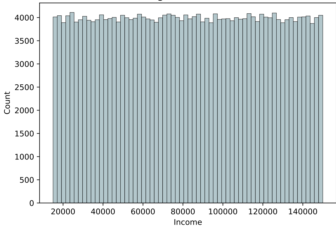
Histogram of Income
