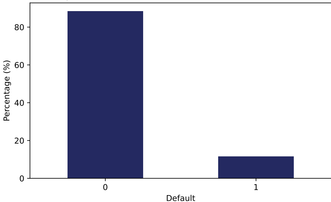
Percentage Distribution of Default - 0: Non-Defaulter, 1: Defaulter
