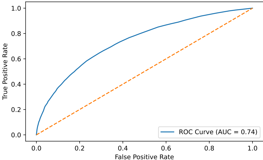
ROC Curve - Loan Default Prediction
