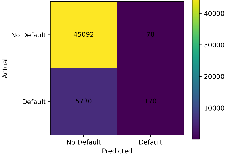
Confusion Matrix - Loan Default Prediction
