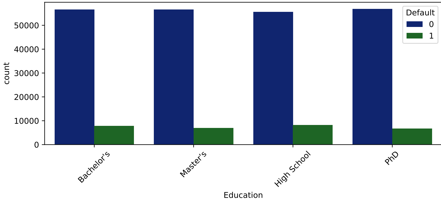
Education Level vs Default - 0: Non-Defaulter, 1: Defaulter'
