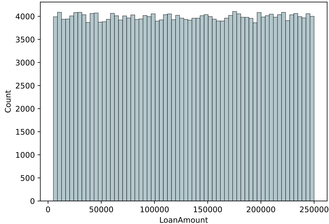
Histogram of LoanAmount
