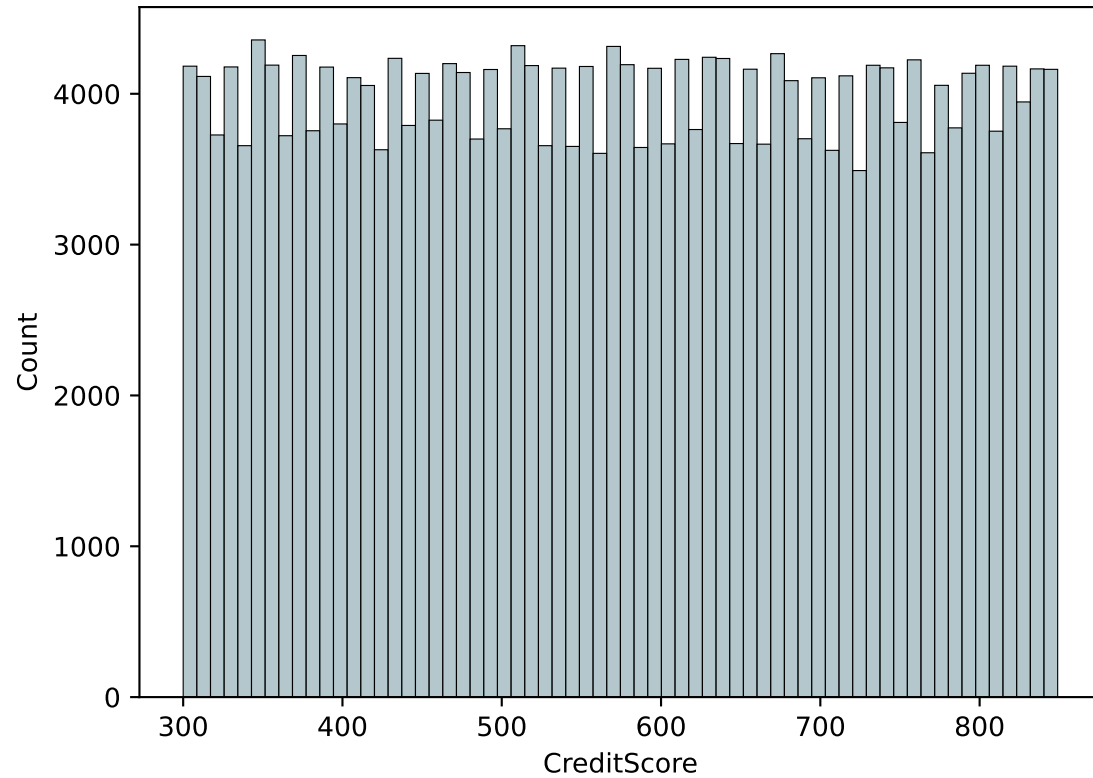
Histogram of CreditScore
