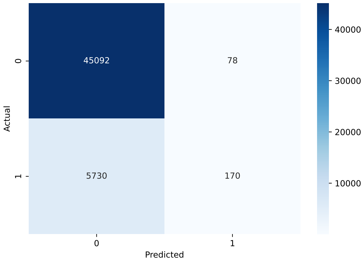
Confusion Matrix - Loan Default Prediction
