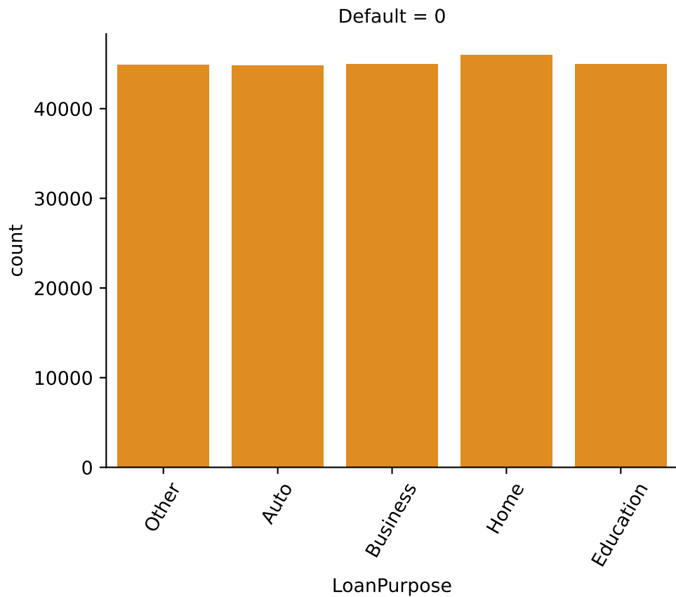
LoanPurpose Distribution of Default - 0: Non-Defaulter, 1: Defaulter
