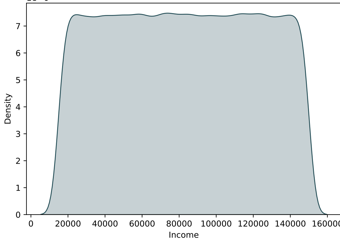
Distribution of Income
