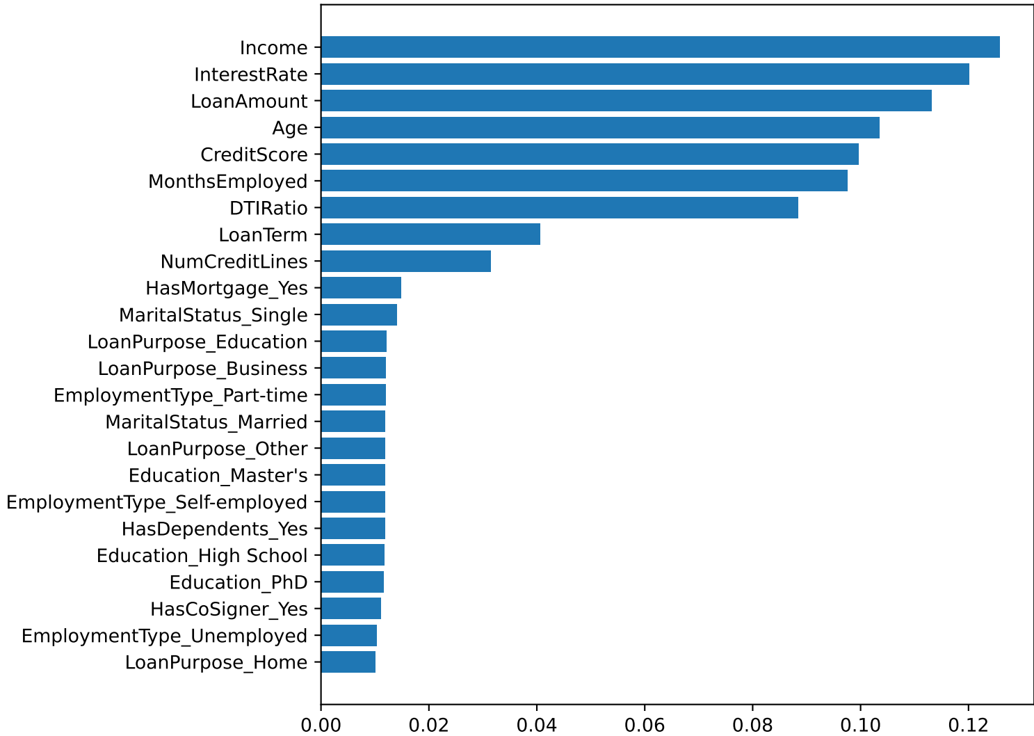
Feature Importance in Credit Risk Prediction
