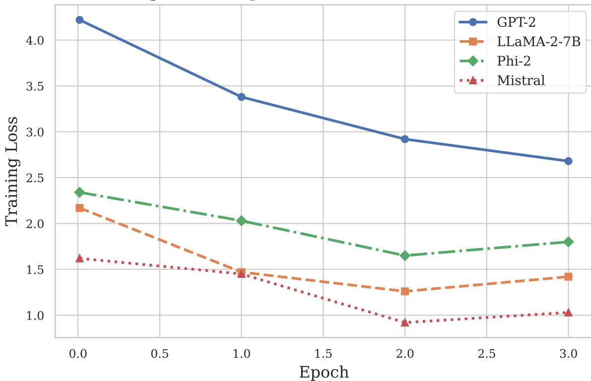
Training Loss Comparison Across Transformer Models
