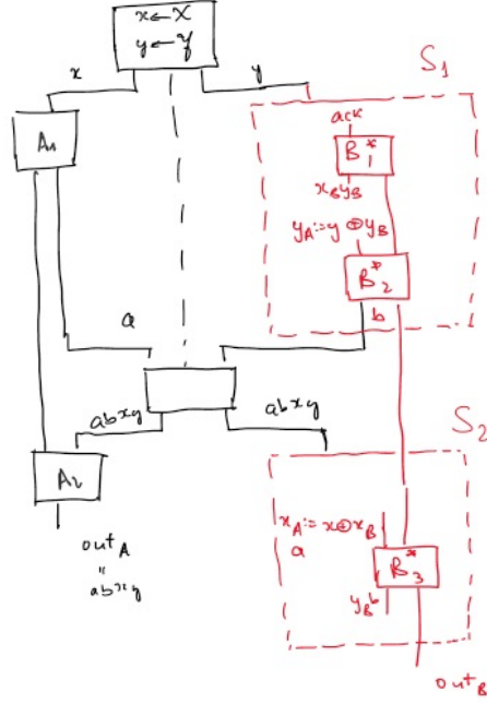
Figure 7: Adversary \mathcal{S} (in red) corrupting party B for protocol \Pi_{\mathcal{F}_{NL}} with input (\square_A, \square_B) . The procedure for \mathcal{S} is decomposed into \mathcal{S}_1 and \mathcal{S}_2
