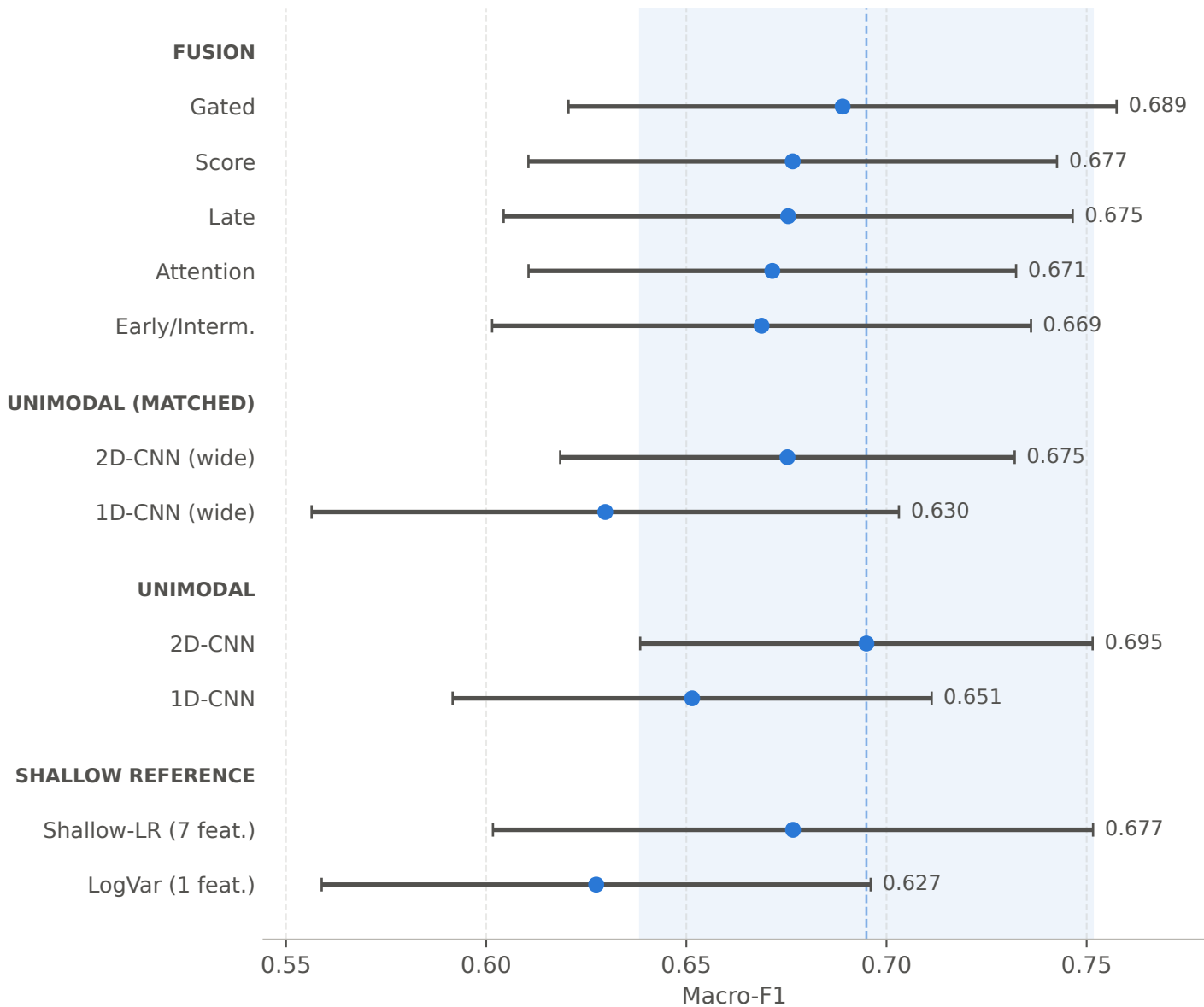
Macro-F1: mean and 95% CI (24 paired measurements) shaded band: CI of the best model
