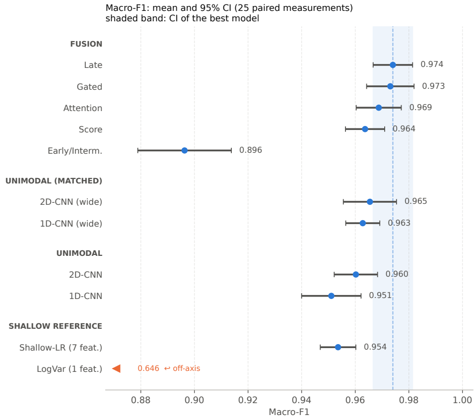
Figure 1: Bonn T1, mean macro F1 with 95% CI per model, grouped by family. Early/intermediate fusion (bold, Table 2) is the one operator visibly separated from the fusion cluster; logvar sits far off axis and is shown pinned to the left edge with its value labelled, rather than compressing the rest of the plot.
