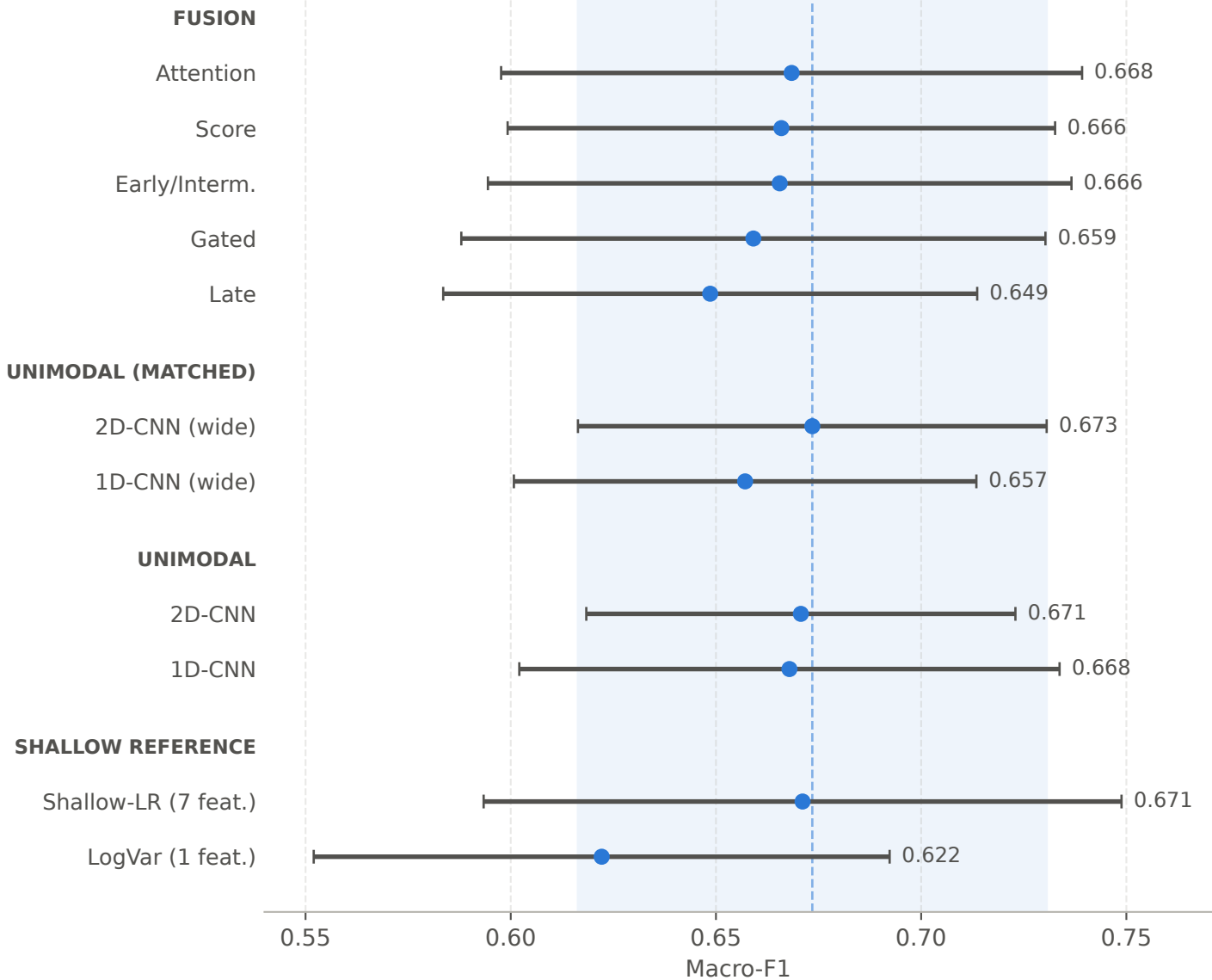
Macro-F1: mean and 95% CI (23 paired measurements) shaded band: CI of the best model
