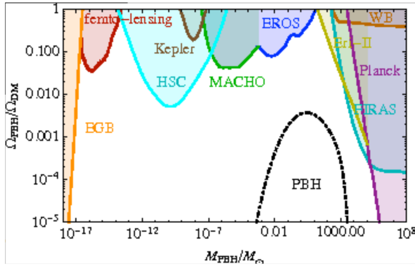
Figure 8.8: Mass of Primordial Black Holes (PBHs) and corresponding constraints on their abundance as dark matter candidates.
