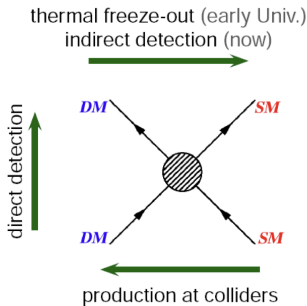
Figure 8.5: The three main methods for non-gravitational detection of dark matter: direct detection, indirect detection, and collider detection.
