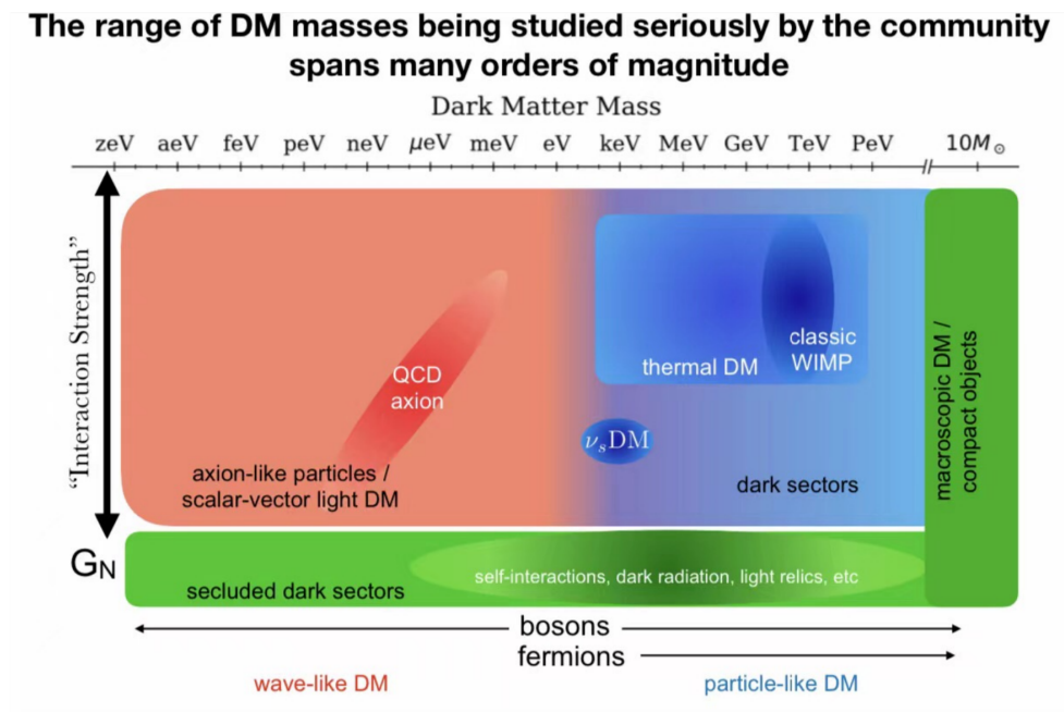
Figure 8.7: Some of the hypothetical candidates for dark matter.
