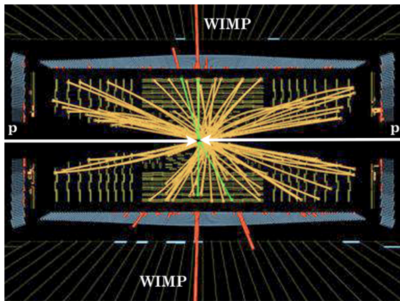
Figure 8.6: A proton-proton collision event in a collider experiment, with potential production of WIMPs (invisible particles) leading to missing transverse momentum.
