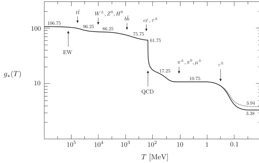
Figure 5.1: Evolution of g_* with temperature.
