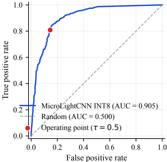
ROC curve — ESD test set
