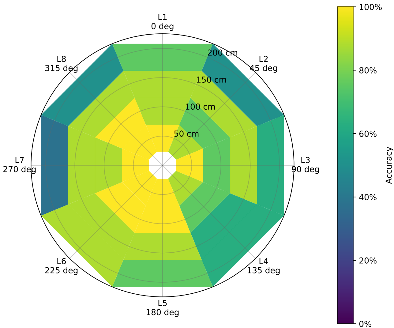
Joint anger and speaker accuracy
