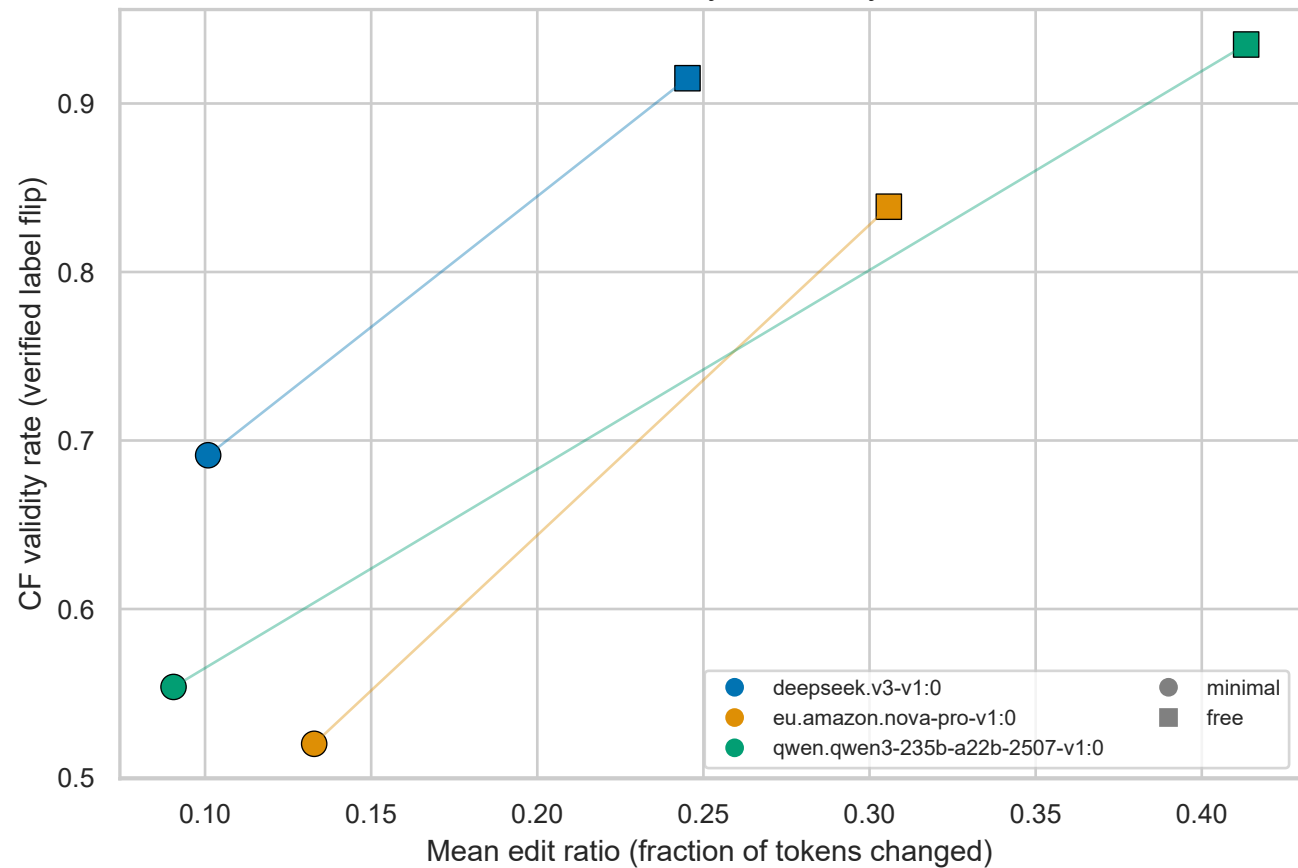
Counterfactual validity–minimality trade-off
