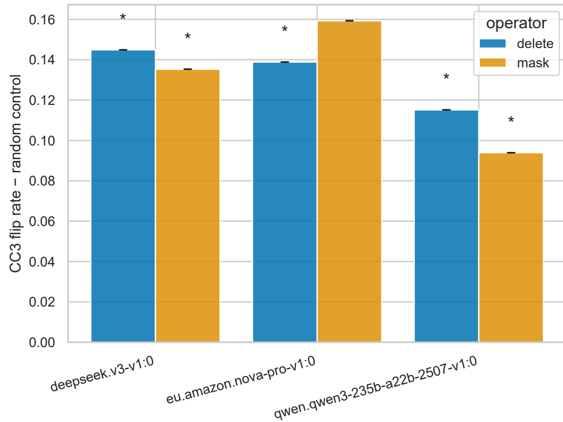
(a) Consensus-core erasure gap (per model)
