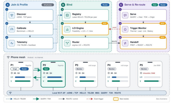
Fig. 3. System Architecture, Functions of Phones within the Local Mesh.
