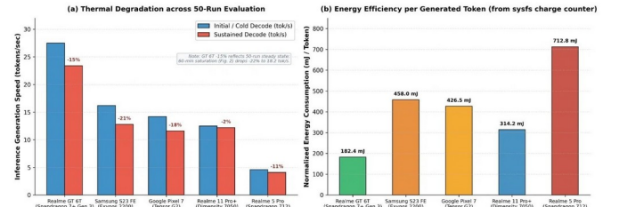
Fig. 4. Thermal Degradation across 50-Run Evaluation and Energy Efficiency per Generated Token.
