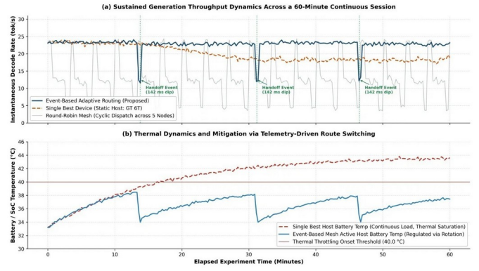
Fig. 5. 60-Minute Throughput and Thermal Dynamics.
