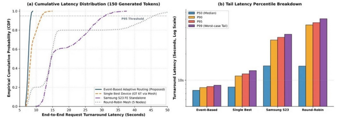
Fig. 6. Latency CDF and Tail Percentiles.
