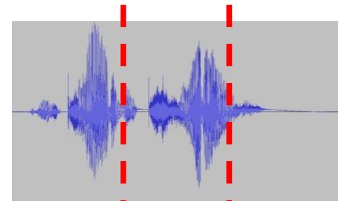
Original Audio
