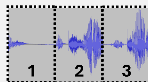
Shuffled Audio
