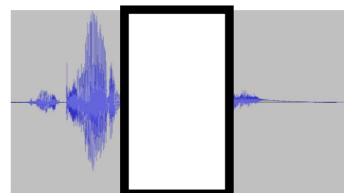
Masked Audio
