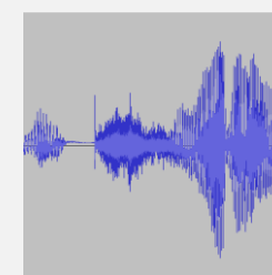
Candidates
