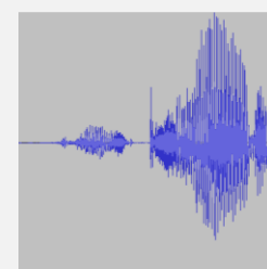
Candidates
