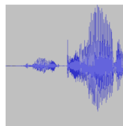
Query
