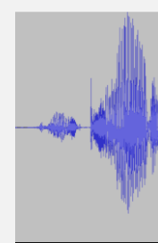
Candidates
