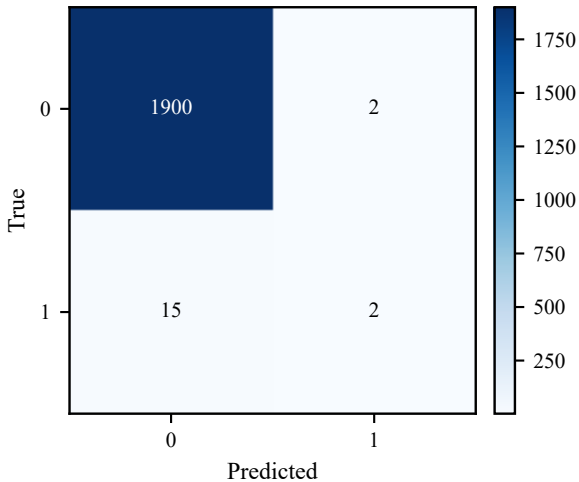
T1 confusion (seed404)
