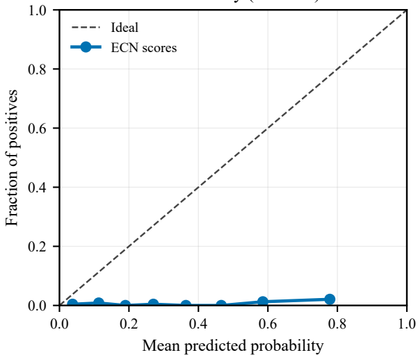
T2 reliability (seed202)
