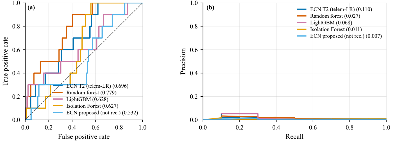
Fig. 9. T2 ROC (a) and precision-recall (b) curves on frozen instance v1.1.0-INST. The recommended T2 operating head is telemetry logistic regression (labeled ECN T2 (telem-LR)); the multi-agent proposed T2 curve is shown only for contrast.
