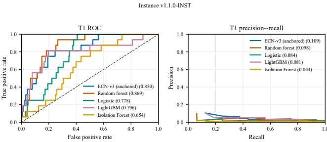
Fig. 4. T1 ROC (left) and precision–recall (right) curves on frozen instance v1.1.0-INST for representative detectors, including the final anchored ECN-v3 head. Legend values report ROC-AUC and average precision on this instance.
