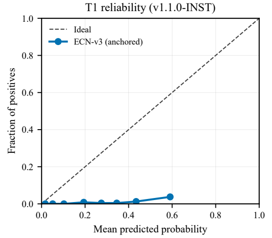
Fig. 7. T1 reliability diagram on instance v1.1.0-INST for the anchored ECN-v3 head. The dashed line denotes perfect calibration. Optional Beta calibration is recommended for operator-facing probabilities.
