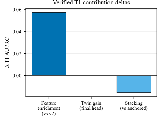
Fig. 6. Verified T1 AUPRC deltas from architecture selection: feature enrichment versus v2, twin gain under the final head, and stacking versus anchored fusion.
