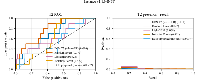
Fig. 9. T2 ROC (left) and precision-recall (right) curves on frozen instance v1.1.0-INST. The recommended T2 operating head is telemetry logistic regression (labeled ECN T2 (telem-LR)); the multi-agent proposed T2 curve is shown only for contrast.
