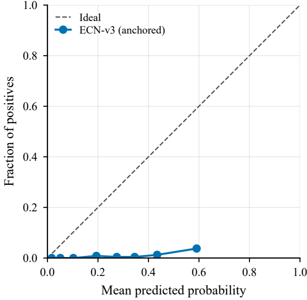
Fig. 7. T1 reliability diagram on instance v1.1.0-INST for the anchored ECN-v3 head. The dashed line denotes perfect calibration. Optional Beta calibration is recommended for operator-facing probabilities.
