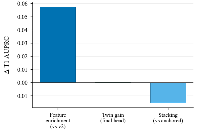
Fig. 6. Verified T1 AUPRC deltas from architecture selection: feature enrichment versus v2, twin gain under the final head, and stacking versus anchored fusion.
