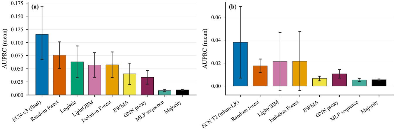
Fig. 3. Multi-seed mean AUPRC with 95% confidence intervals. (a) T1 anomaly detection, where ECN-v3 denotes the final anchored head on enriched features. (b) T2 failure-horizon ranking; the ECN T2 column is the recommended telemetry logistic head.
