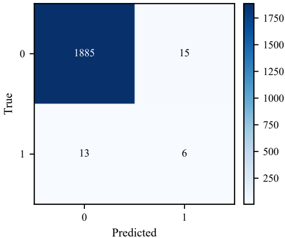
T1 confusion (seed202)
