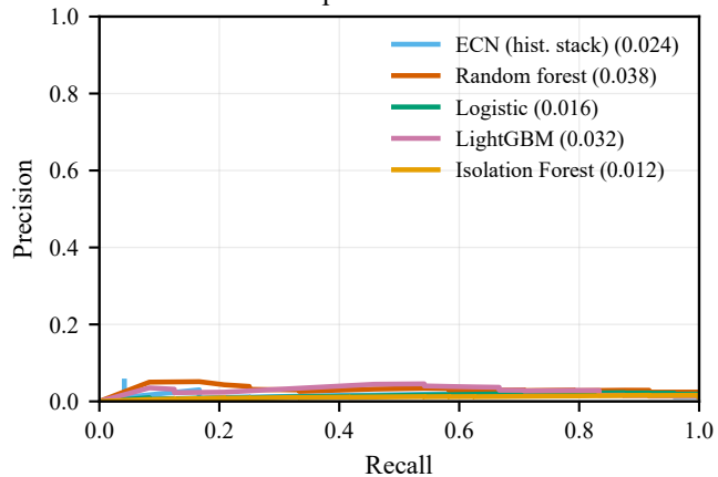
T1 precision--recall
