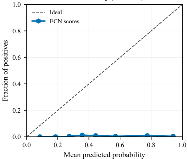
T2 reliability (seed303)
