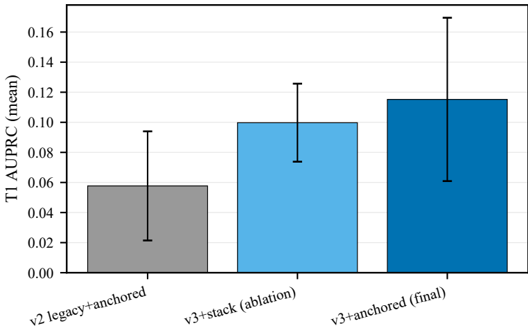
Feature/fusion ablation (T1)
