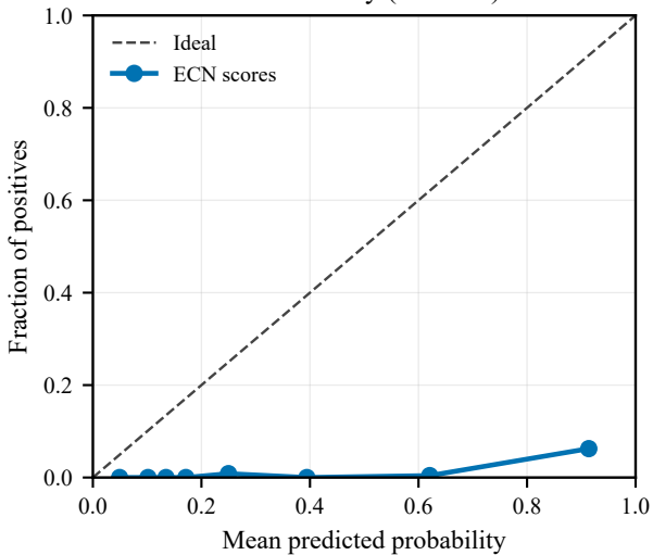
T1 reliability (seed101)
