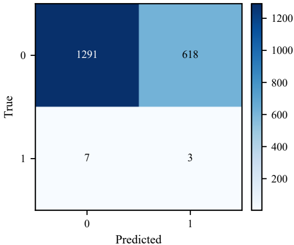
T2 confusion (seed303)
