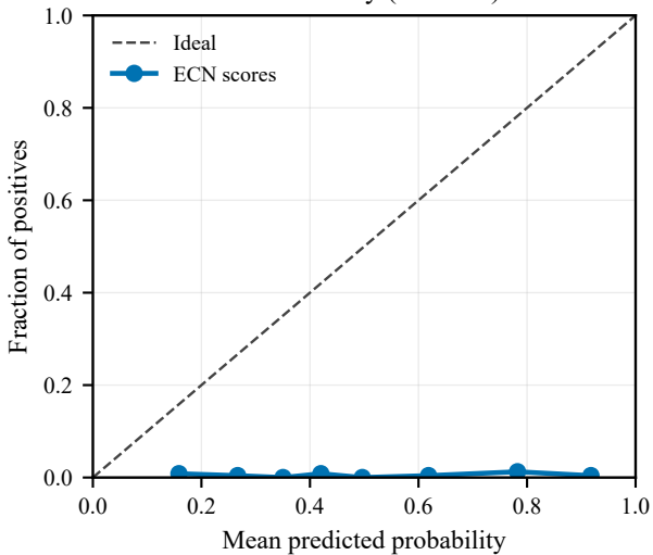
T2 reliability (seed404)
