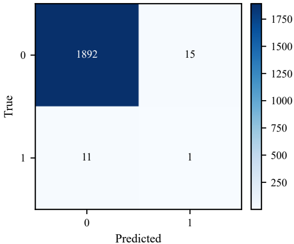
T2 confusion (seed505)
