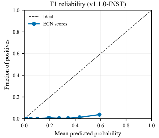
Fig. 7. T1 reliability diagram on instance v1.1.0-INST. The dashed line denotes perfect calibration. Optional Beta calibration is recommended for operator-facing probabilities.
