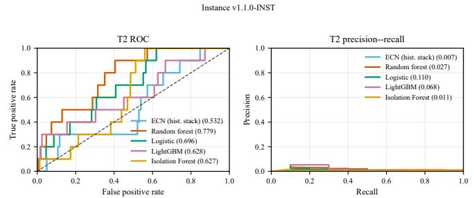
Fig. 9. T2 ROC (left) and precision-recall (right) curves on frozen instance v1.1.0-INST. The recommended T2 operating head is telemetry logistic regression.
