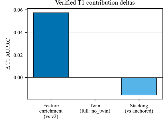
Fig. 6. Verified T1 AUPRC deltas: feature enrichment versus v2, twin contribution under the final head, and stacking versus anchored fusion.
