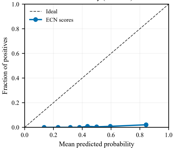
T2 reliability (seed101)
