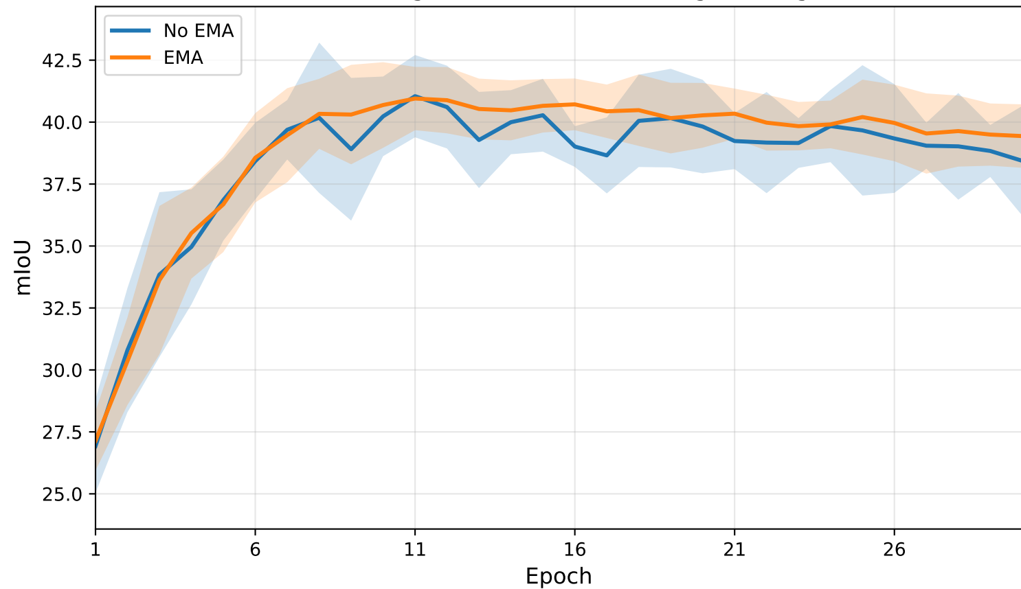
BDD: Target-Domain mIoU During Training
