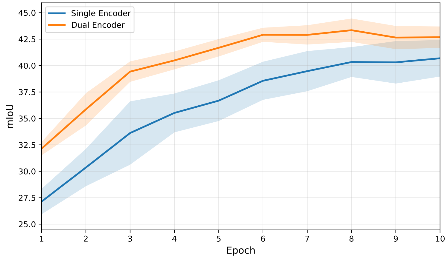
Early target-domain performance: BDD / EMA
