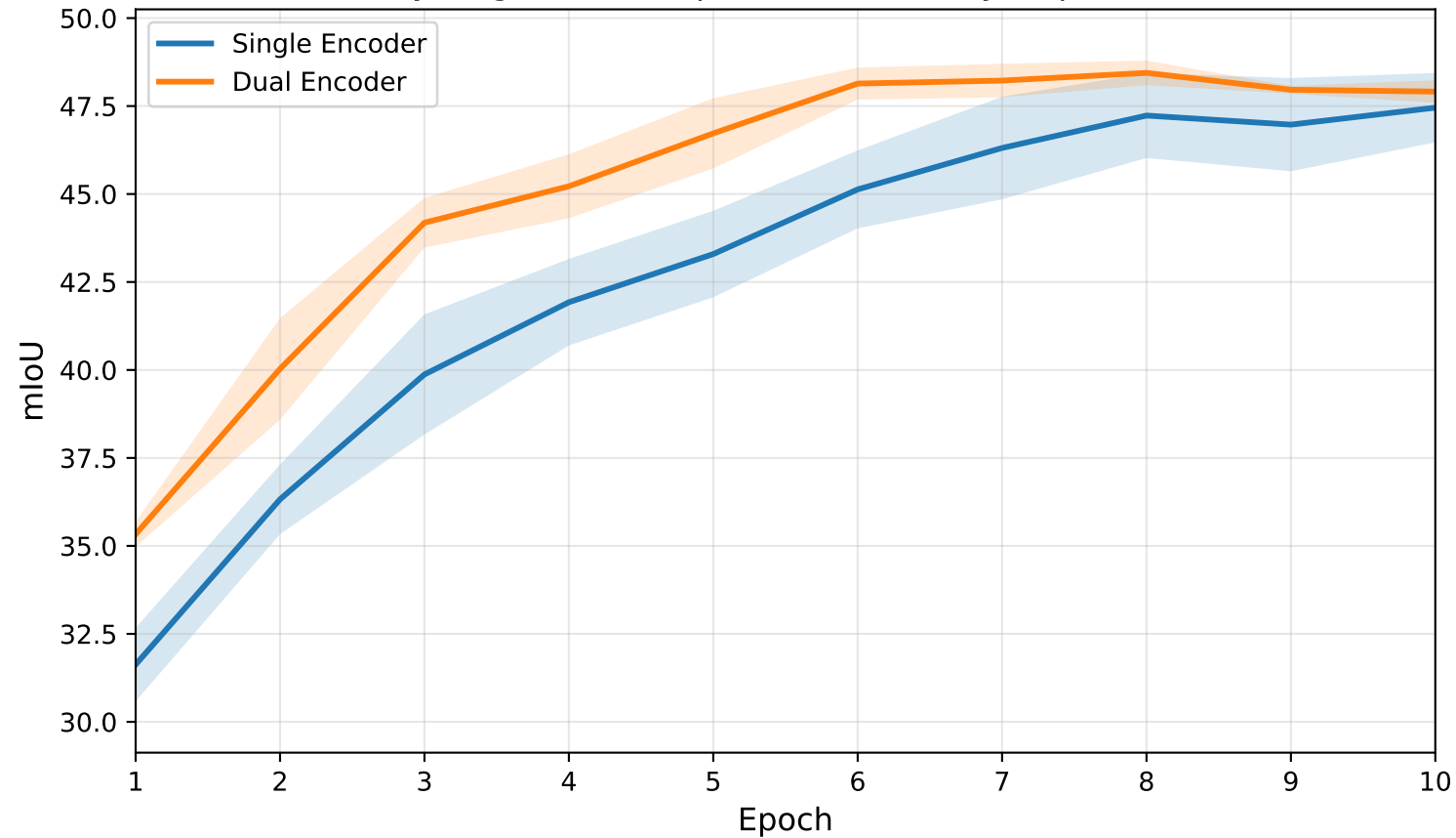
Early target-domain performance: Cityscapes / EMA
