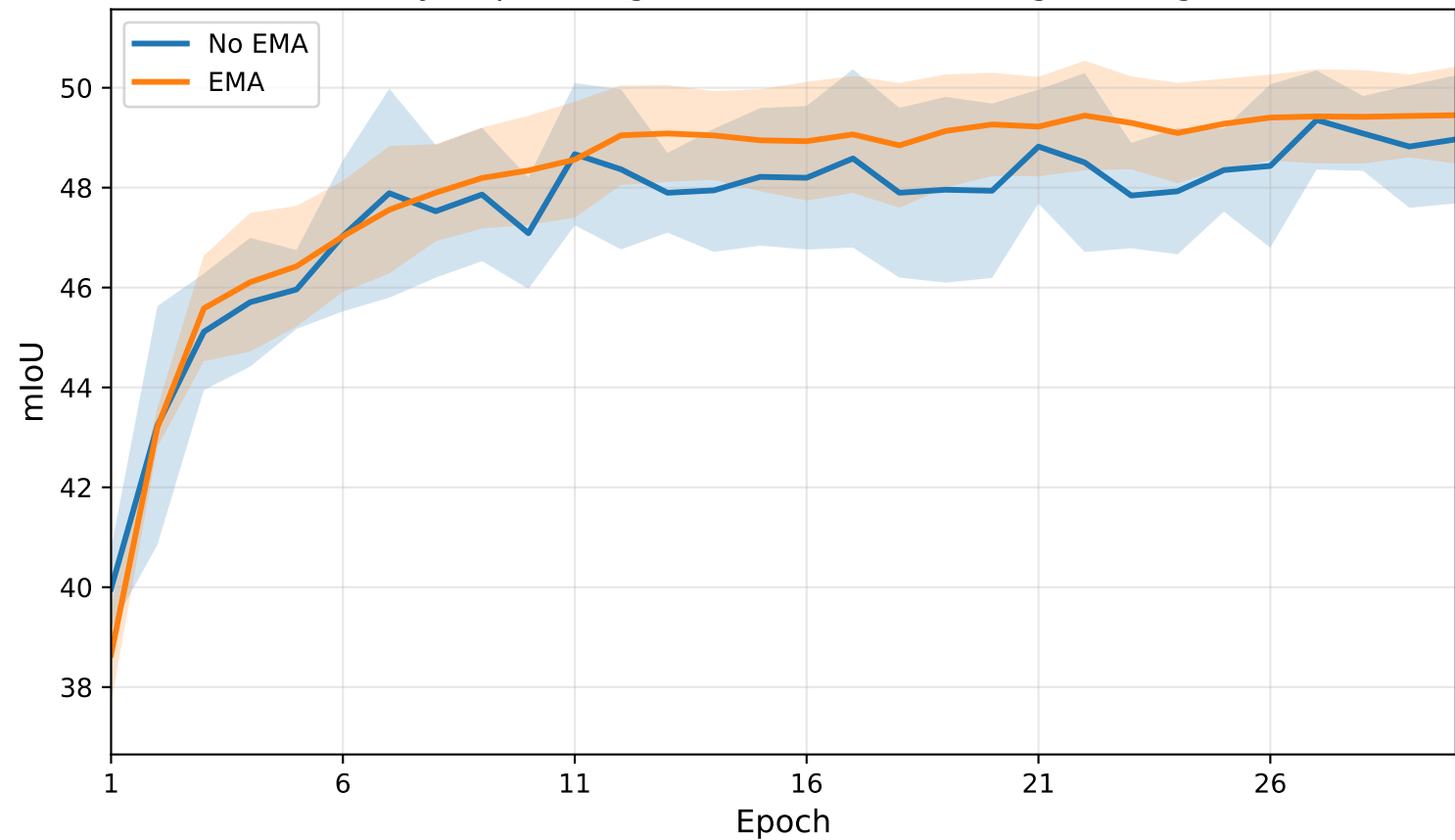
Cityscapes: Target-Domain mIoU During Training
