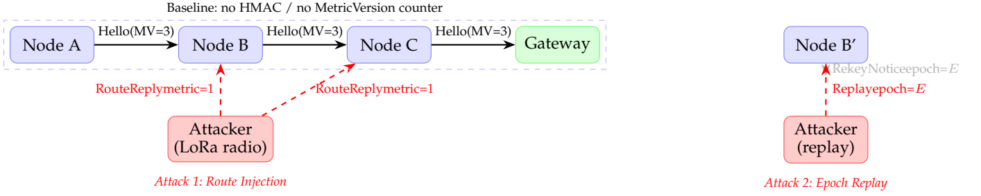
Fig. 1. LoRaMesher IoT mesh attack surface. Left : Route-injection attack — attacker broadcasts forged RouteReply ( metric=1 ) to redirect all traffic through itself. Right : Replay attack — replayed RekeyNotice ( epoch=E ) confuses nodes into a stale session epoch. Both attacks require only a commodity LoRa transceiver ($18–50).
