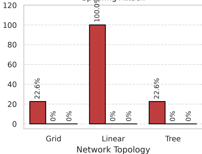
Spoofing Attack
