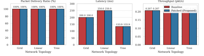
Fig. 5. Network performance metrics under normal operation. The security patches maintain 100% PDR and constant throughput with minimal latency impact.
